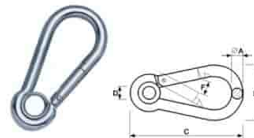
DR-Z0019 SNAP HOOK WITH EYELET DIN 5299 FORM A
