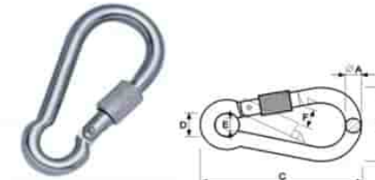
DR-Z0020 SNAP HOOK WITH SCREW DIN 5299 FORM D
