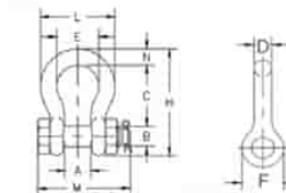
DR-Z0052 G2130 BOLE TYPE ANCHOR SHACKLES
