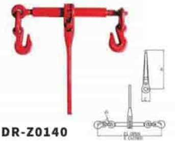
LOAD BINDER RABBIT
